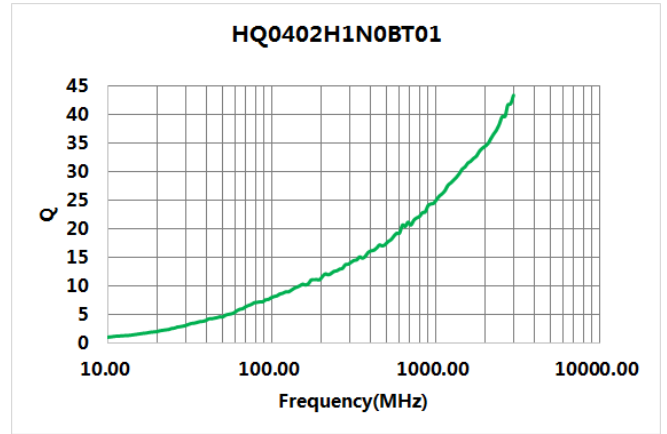
Q-Frequency Characteristics(Typ.)
